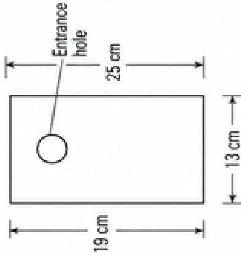
4. Front panel
